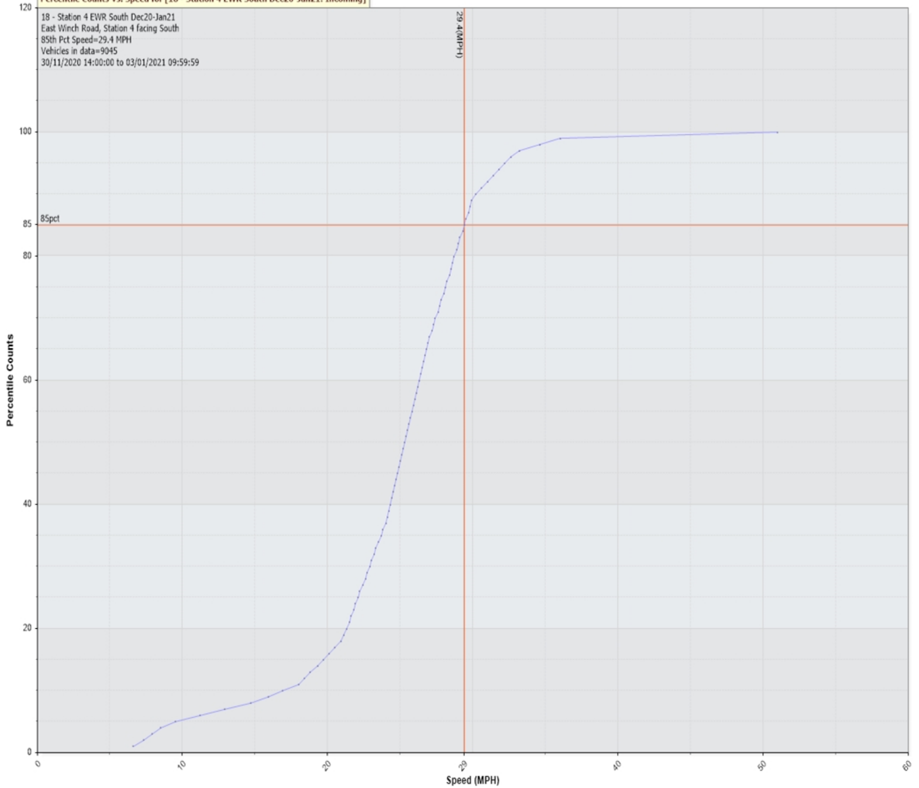
Percentile Counts Vs. Speed for [18 - Station 4 EWR South Dec20-Jan21: Incoming]
